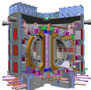
ITER graphical cut. Courtesy of ITER
